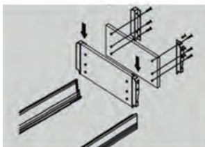
Railing installation
