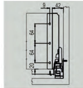
Back fixing brackets position
