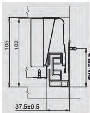
Cabinet dimension
