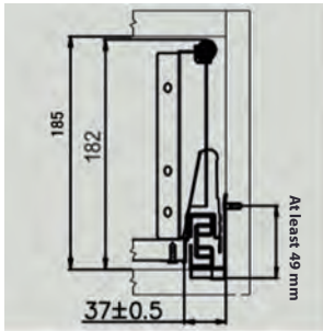
Installation of front fixing brackets
