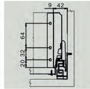
Back fixing brackets position
